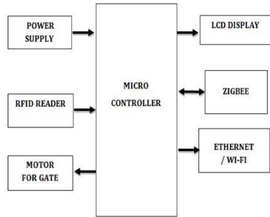
Fig: Security Section Block Diagram
